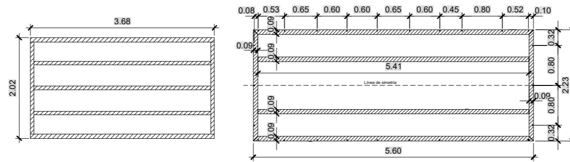
FOOTPRINT LAYOUT
